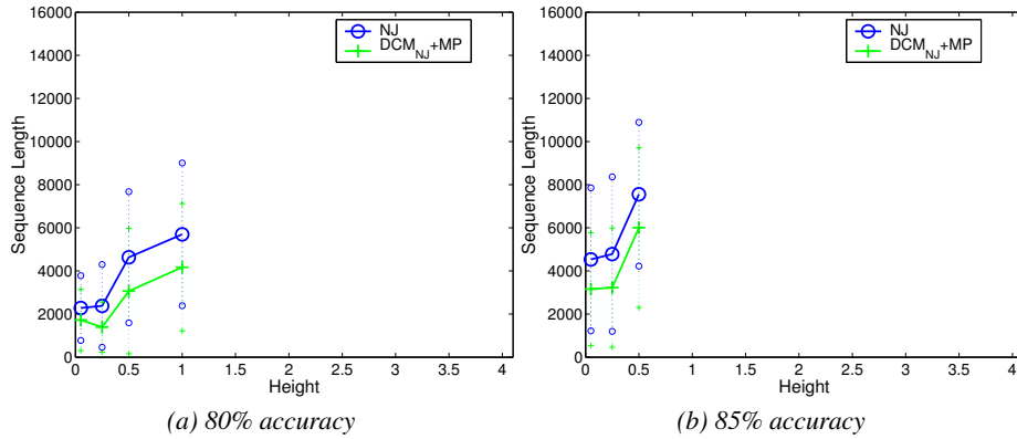
Fig. 3. Sequence-length requirements as a function of the height of the tree, for an expected deviation of 2.02, 100 taxa, and two levels of accuracy.
