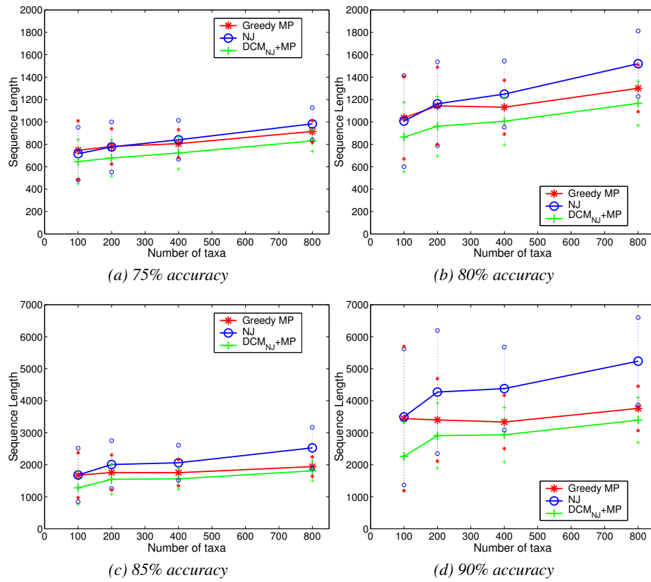
Fig. 4. Sequence-length requirements as a function of the number of taxa, for an expected deviation of 1.36, a height of 0.05, and four levels of accuracy.
