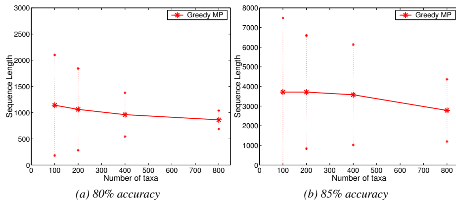
Fig. 5. Sequence-length requirements for Greedy MP (60 runs) as a function of the number of taxa, for an expected deviation of 1.36, a height of 0.5, and two levels of accuracy.
